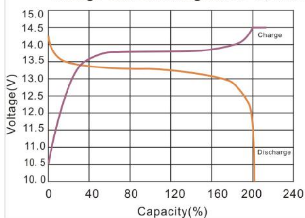
Charge and Discharge at 25°C, 0.2C
